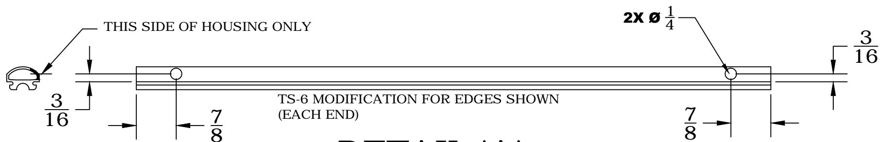
DETAIL 'A'
