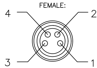
22AWG/4, PVC JACKETED (M8), FEMALE:
