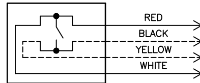
TYPICAL CKP/AMCKP 4-WIRE STANDARD CABLE ANALOGUE:
