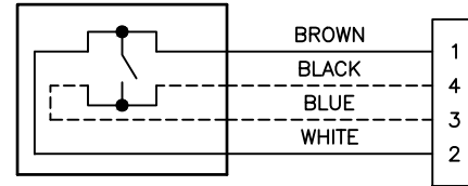
22AWG/4, PVC JACKETED (M8), MALE:
