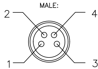
22AWG/4, PVC JACKETED (M8), MALE:
